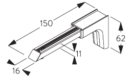
SG 11155 Universal Smart Fix 150 mm
